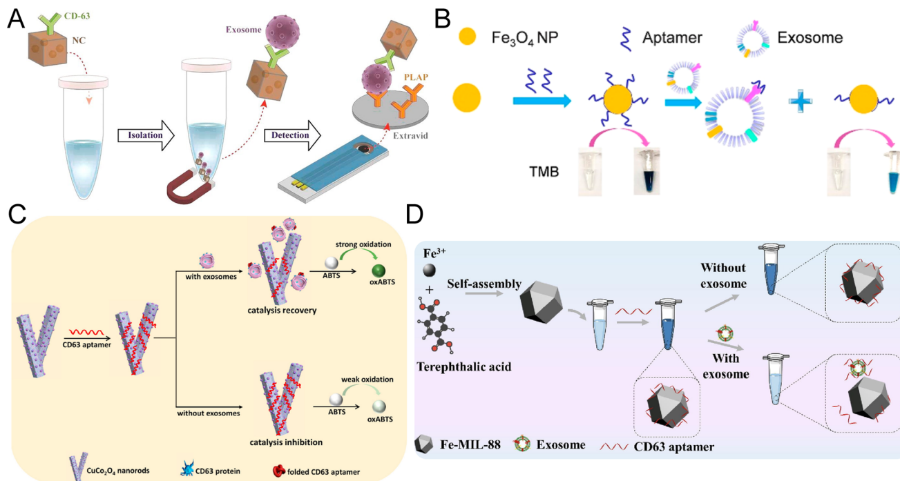
Fig. 5 Colorimetric biosensors developed based on magnetic nanomaterials and metal–organic frameworks. (A) Au-NP/Fe 3 O 4 NCs were applied as detection probes and enabled the direct isolation of exosomes. The complex was transferred to antibody-coated electrodes for the formation of a typical sandwich structure. Reproduced from ref. 91 with permission from the American Chemical Society, copyright 2019. (B) Fe 3 O 4 -NP-based competitive reaction for the detection of exosomes isolated through the anion exchange mechanism. Reproduced from ref. 90 with permission from the American Chemical Society, copyright 2018. (C) Colorimetric biosensor based on the release of CD63 aptamers from the CuCo 2 O 4 nanorod surface in the presence of exosomes, resulting in the recovery of catalytic activity. Reproduced from ref. 98 with permission from Elsevier, copyright 2021. (D) Application of MOF nanozymes in a one-step reaction based on the regulation of Fe-MOFs through ssDNA. Reproduced from ref. 99 with permission from Elsevier, copyright 2022.
