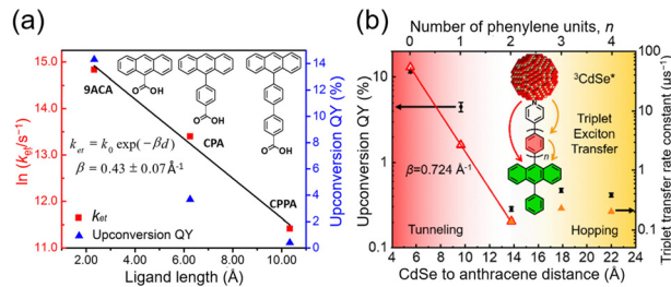
Fig. 7 Distance dependence of the TET rate constant and UC efficiency in (a) CdSe:X/DPA ( X = 9\text{-ACA, CPA, CPPA} ) and (b) CdSe:PyPxPAN/DPA ( x = 0-4 ) systems. Reproduced from ref. 41 with permission from Journal of American Chemical Society, Copyright 2016 and ref. 42 with permission from American Chemical Society, Copyright 2020.
