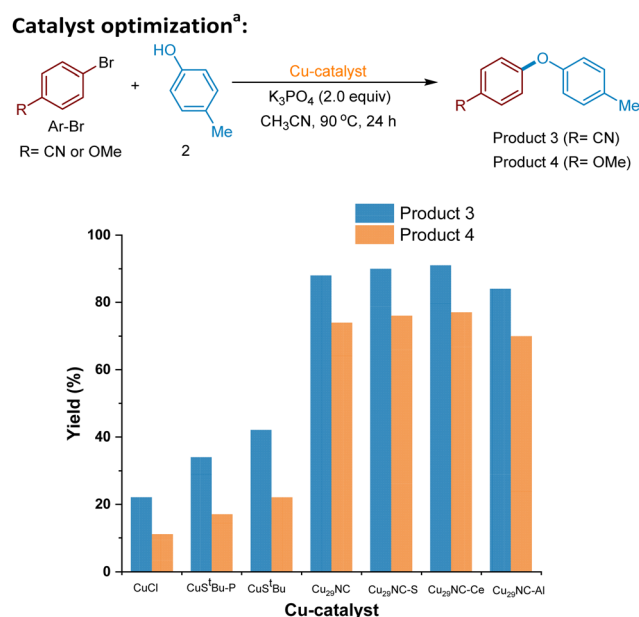
Fig. 4 Catalyst optimization. a Conditions: Ar–Br (0.3 mmol), 2 (0.375 mmol), Cu-catalyst used such as 5 mol% of CuCl or Cu t S t Bu-PPh 3 , Cu t S t Bu or 0.025 mol% of Cu 29 NC or Cu 29 -Celite S or Cu 29 NC-CeO 2 or Cu 29 NC-Al 2 O 3 , K 3 PO 4 (2.0 eq.), and acetonitrile (CH 3 CN) (2 mL). The mixture was stirred at 90 °C for 24 h. Yield refers to GC yield using 1,3,5-trimethylbenzene (mesitylene) as the internal standard.
