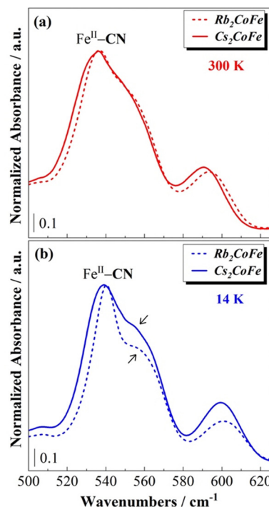
Fig. 6 Spectra of \text{Rb}_2\text{CoFe} and \text{Cs}_2\text{CoFe} over the 500\text{--}620\text{ cm}^{-1} range at (a) 300 K and (b) at 14 K.
