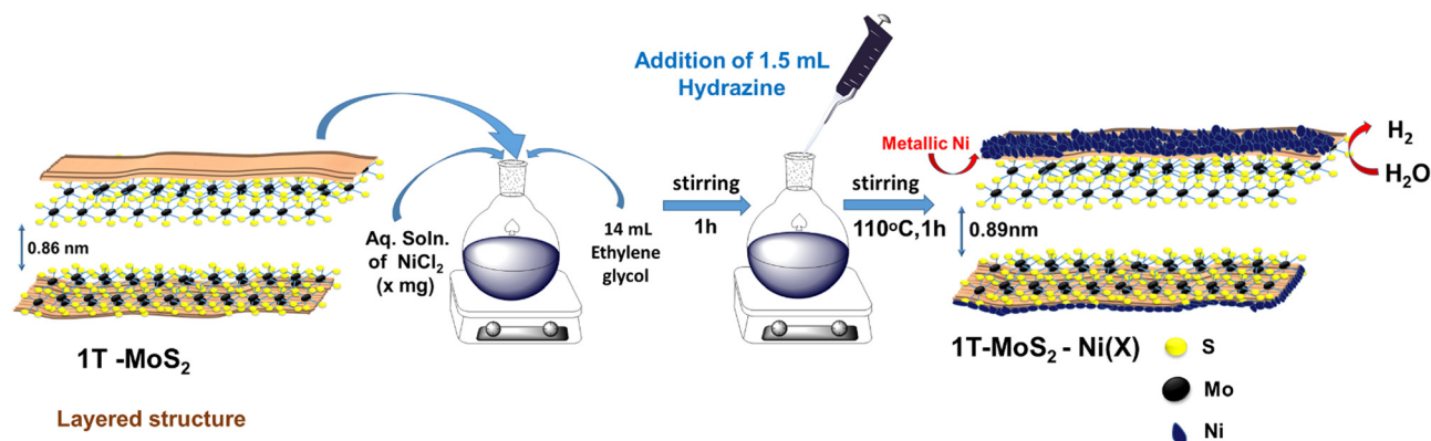
Fig. 1 Schematic representation of the synthetic protocol to prepare the 1T-MoS 2 -Ni(X) composite structure.
