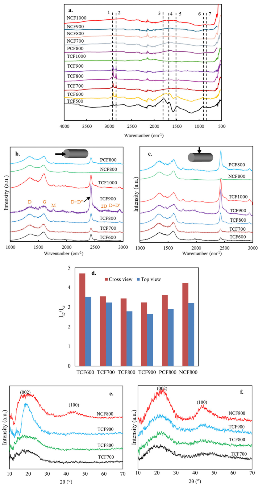
Fig. 8 Characterization of 100% OL-derived CFs. (a) FTIR spectra: 1 (2914 \text{cm}^{-1} ) & 2 (2850 \text{cm}^{-1} ) for alkyl C–H stretch, 3 (1760 \text{cm}^{-1} ) & 4 (1650 \text{cm}^{-1} ) for C=O, 5 (1500 \text{cm}^{-1} ), 6 (913 \text{cm}^{-1} ), and 7 (833 \text{cm}^{-1} ) for aromatic ring vibration. (b–d) Raman spectra: (b) cross-section view spectra; (c) top view spectra; (d) I_D/I_G ratios of CFs in different fiber directions after Gaussian fitting; (e & f) XRD equatorial scans measured at (e) parallel and (f) perpendicular to the fiber axis.
