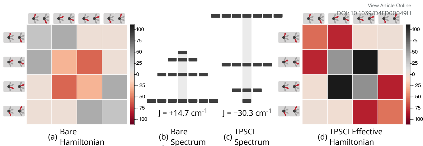
FIG. 6. Bare and Bloch Effective Hamiltonians for \text{Cr}_2(\text{III}) complex. (32e, 38o) active space. Units of J in \text{cm}^{-1} . (a) Hamiltonian matrix in the basis of M_s = 0 tensor products of local spin states where all the bridging ligands are in singlet states, and the Cr centers are in |S = \frac{3}{2}, M_s = \pm \frac{3}{2}\rangle (b) Energy spectrum of bare Hamiltonian in local S = \frac{3}{2} basis. (c) Energy spectrum of extrapolated TPSCI results. (e) Bloch Effective Hamiltonian obtained by projecting TPSCI wavefunctions onto local S = \frac{3}{2} basis.
