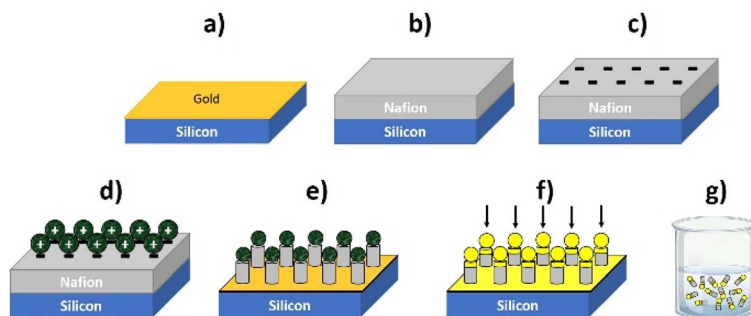
Fig. 4 Different steps in the nanofabrication process: (a) a thin layer deposition of Au on SiO 2 wafers, (b) spin coating of Nafion films (followed by heating at 100 °C for 2 minutes), (c) and (d) electrostatic self-assembly of positive colloidal particles as RIE masks taking advantage of the negative charge of Nafion films, (e) O 2 RIE to define the Nafion pillars, (f) directional metal/oxide evaporation to confer more functionality to the Nafion pillar arrays and reinforce the pillar robustness and (g) release of the Nafion structures into water with an ultrasonic bath.
