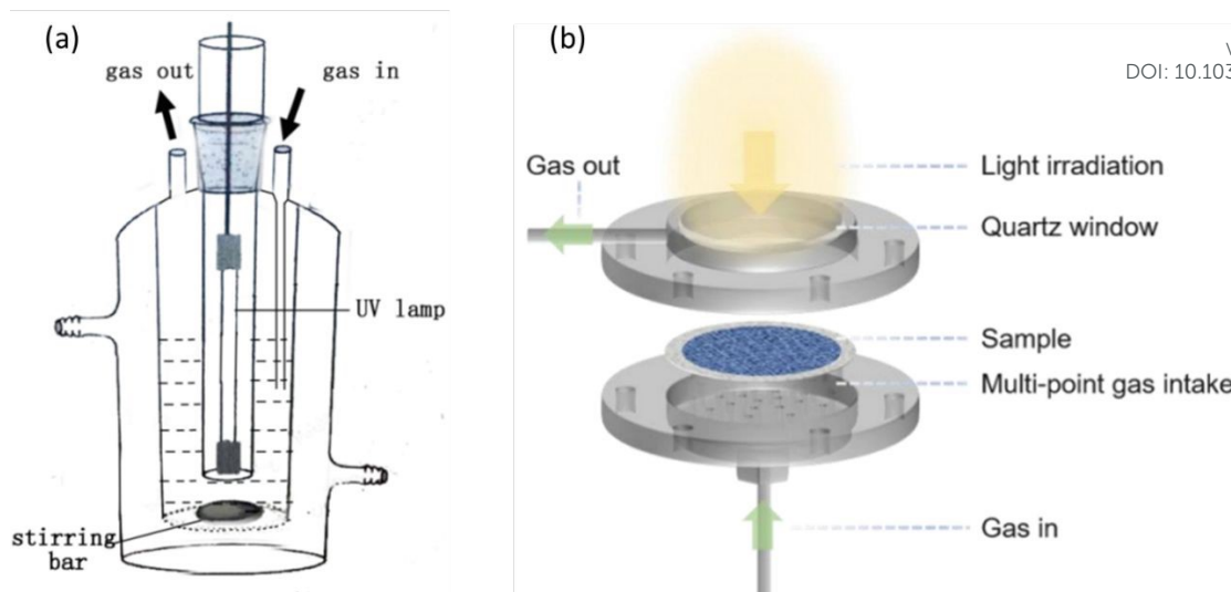
Figure 15. Schematic representation of photocatalytic methane conversion in (a) batch reactor; Reproduced with permission. 71 Copyright 2016, Elsevier. (b) flow reactor. Reproduced with permission. 104 Copyright 2024, American Chemical Society.
