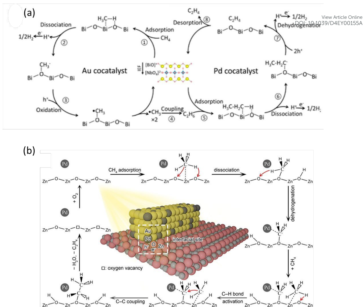
Figure 14. Schematic representation of photocatalytic NOCM to C_2H_4 reaction mechanisms over (a) Au-Pd/BiNbO 5 F; Reproduced with permission. 76 Copyright 2023, American Chemical Society. (b) AuPd/ZnO. Reproduced with permission. 73 Copyright 2020, American Chemical Society.
