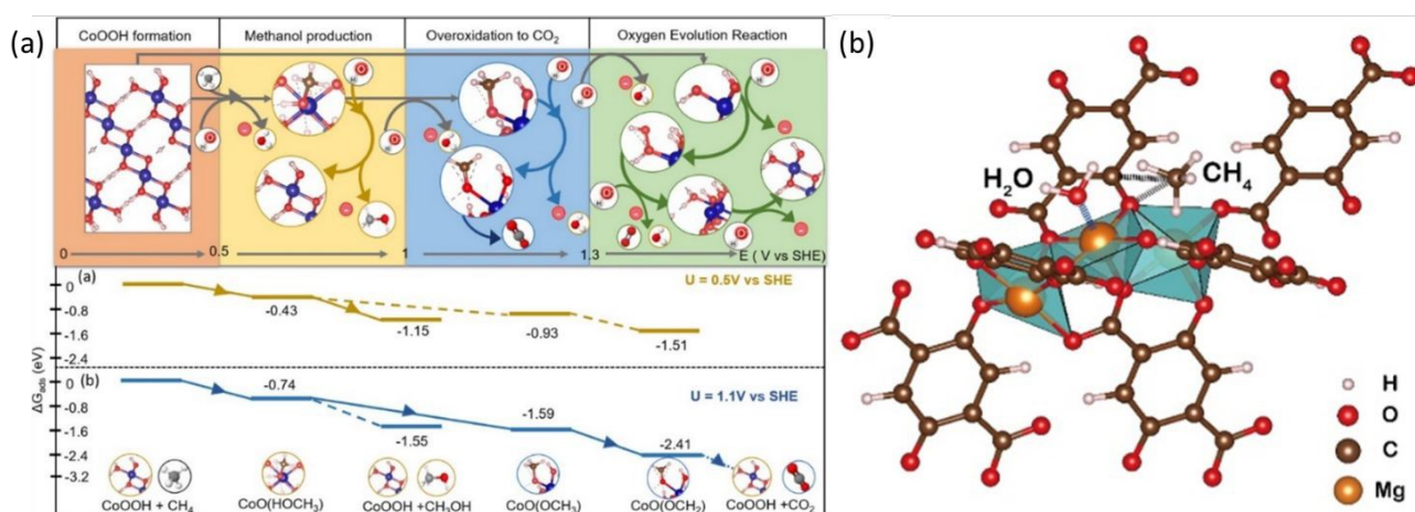
Figure 6. (a) Reaction mechanism and reaction energy diagram at (a) U = 0.5\text{ V vs SHE} and (b) U = 1.1\text{ V vs SHE} . Top panel shows the favoured reactions at certain electrochemical potential range evaluated at \text{pH} = 12 . Reproduced with permission. 38 Copyright 2023, American Chemical Society. (b) Graphical illustration of the \text{CH}_4 adsorption on Mg-oxo-Mg and \text{H}_2\text{O} adsorption on Mg of Mg-MOF-74. Reproduced with permission. 47 Copyright 2022, Elsevier.
