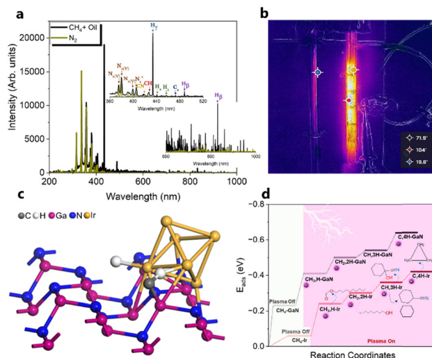
Fig. 8 (a) In situ OES spectra acquired during the plasma driven pyrolysis oil upgrading reaction with \text{CH}_4 over the Ir/GaN catalyst and \text{N}_2 spectra for subtracting the detected strong \text{N}_2 bands. (b) Temperature of the plasma reaction measured using an IR thermal camera. (c) Possible structure and adsorption of CH and H species on the Ir(110) nanoclusters supported on GaN. (d) Adsorption energy diagram and proposed reaction pathway of plasma driven pyrolysis oil upgrading with \text{CH}_4 using the Ir/GaN catalyst.
