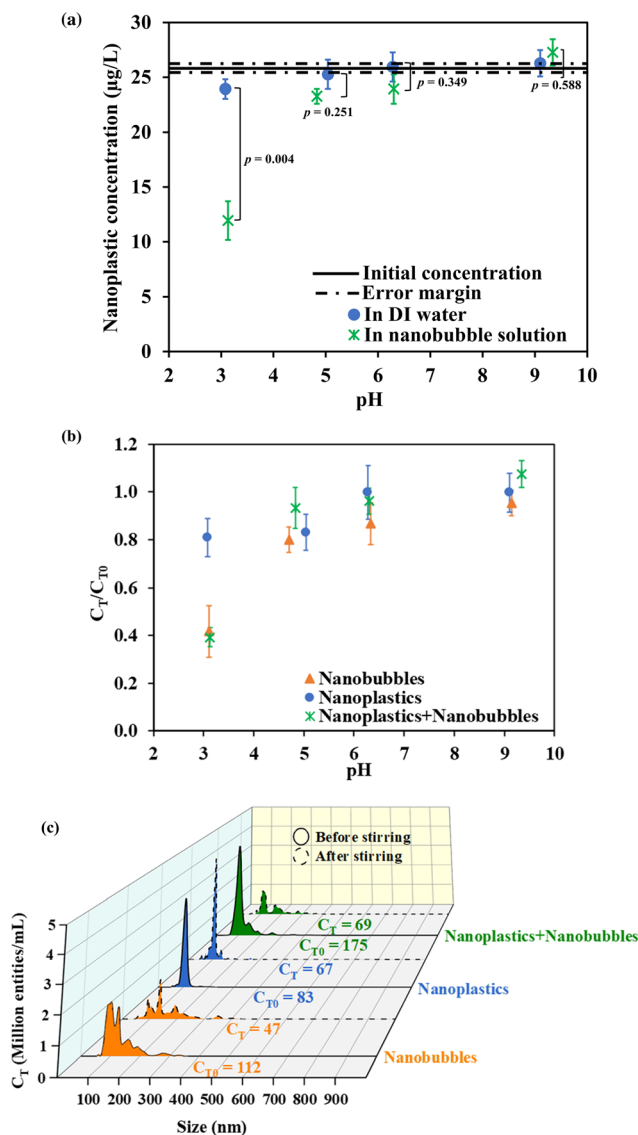
Fig. 1 (a) Nanoplastic concentration in the supernatant after stirring at various pH (conditions: initial nanoplastic concentration = 26 \mu\text{g L}^{-1} , stirring speed = 400 rpm, stirring time = 5 min). The p -values show a statistically significant difference in NP concentration in nanobubble solution vs. DI water. NTA analysis of nano-entities in the supernatant before and after stirring: (b) normalized number concentration at all pH ranges and (c) particle size distributions at pH 3.0. C_{T0} and C_T denote the initial and final number concentration, respectively.
