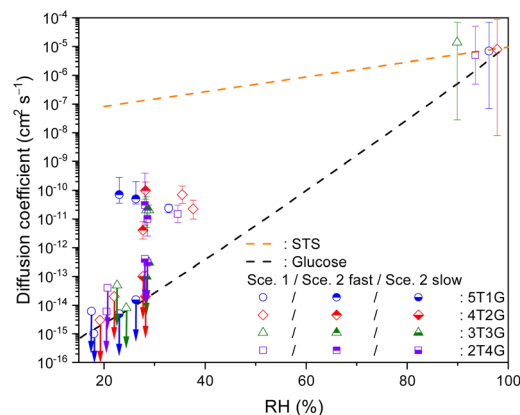
Fig. 5 Bulk diffusion coefficients of \text{S}_2\text{O}_3^{2-} (symbols) in ternary STS:glucose microdroplets at different RHs, as well as the SE predictions for binary STS–water systems and for binary glucose–water systems (lines). 5T1G (blue circles), 4T2G (red diamonds), 3T3G (green triangles) and 2T4G (purple squares): ternary STS:glucose mixtures in mass ratios of 5:1, 4:2, 3:3 and 2:4, respectively. Hollow symbols: D_{b,T} retrieved via Scenario 1. Hollow symbols marked with downward arrows: upper limits of D_{b,T} retrieved via Scenario 1. Top-filled symbols: D_{b,T,fast} retrieved via Scenario 2. Bottom-filled symbols marked with downward arrows: upper limits of D_{b,T,slow} retrieved via Scenario 2. For clarity, the error bars of RH ( \sim 3.5\% ) are not plotted here. The error bars of diffusion coefficients represent the fitting errors for each kinetics data. See Tables S3 and S4† for the full details of diffusion coefficients.
