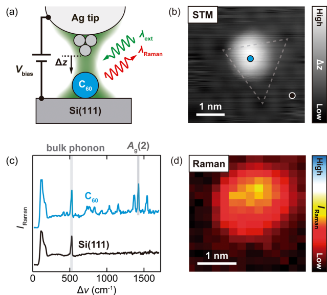
Fig. 1 (a) Schematic of the experimental configuration: a single C 60 molecule junction is formed in the STM junction consisting of the reconstructed Si(111)-(7 × 7) substrate and an Ag tip. (b) STM image of a single C 60 molecule on the Si(111)-(7 × 7) surface, scanned under illumination with the faulted region highlighted with a grey triangle (80 K, V_{\text{bias}} = 0.3 V, j_{\text{STM}} = 60 pA, \lambda_{\text{ext}} = 532 nm, P = 5 mW). (c) TERS spectra recorded over the individual C 60 (blue) and over the bare Si surface (black) acquired on the points depicted in (b) (averaging time = 5 s). (d) TERS map of the Ag g (2) peak (80 K, feedback on, setpoint: V_{\text{bias}} = 0.3 V and j_{\text{STM}} = 50 pA, \lambda_{\text{ext}} = 532 nm, P_{\text{ext}} = 5.5 mW, 16 × 14 pixels, 5 s per point, TERS scale bar: arbitrary units).
