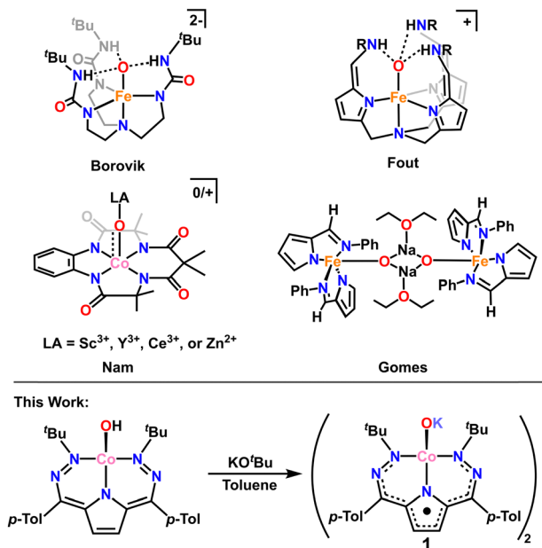
Scheme 1 Top: Examples of previously reported metal oxides stabilized by hydrogen bonding or Lewis acid interactions. Bottom: Synthesis of 1 from [\text{t}^{\text{Bu}},\text{ToI}]\text{DHP}[\text{CoOH}] .
