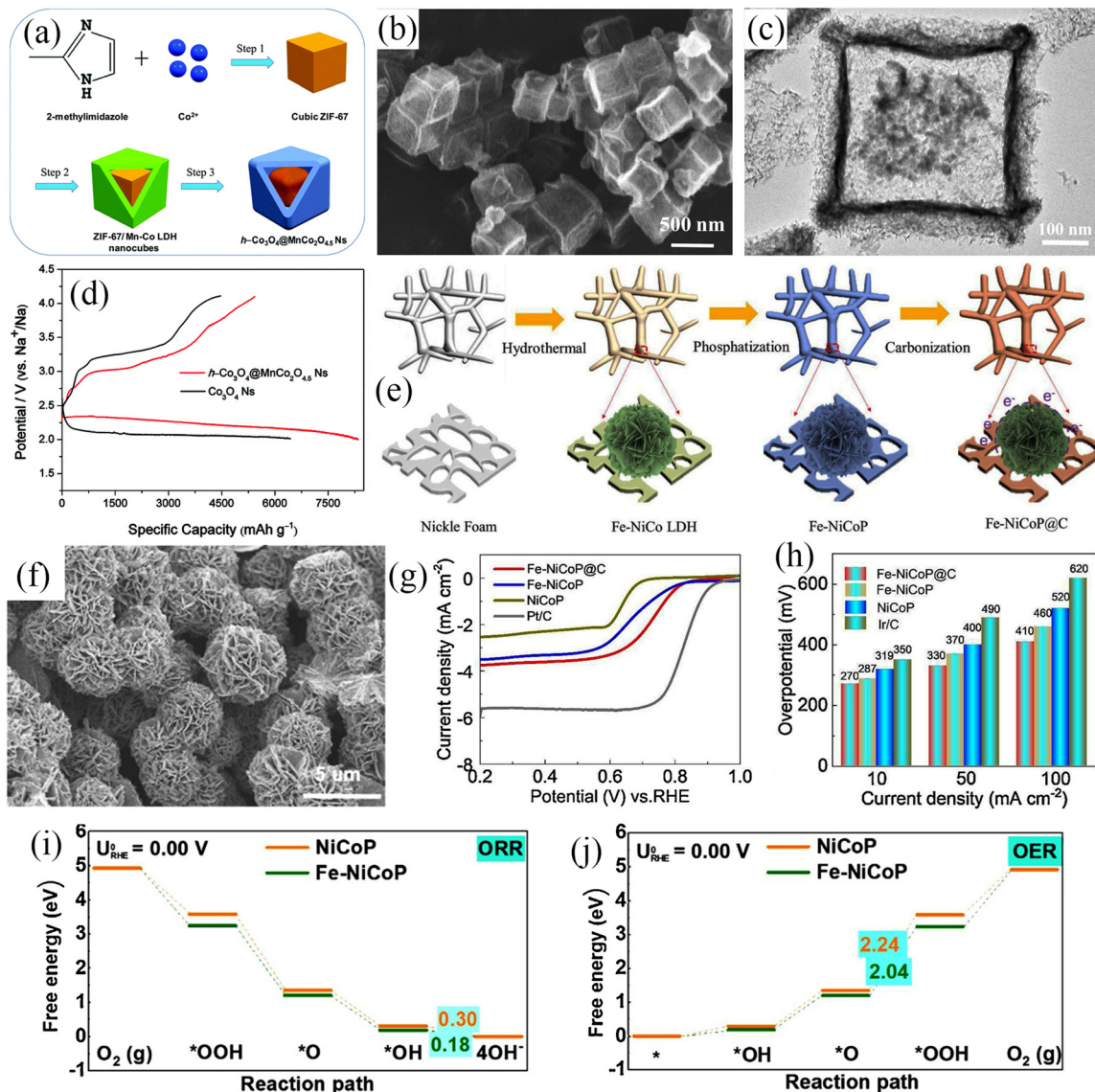
Fig. 17 (a) Scheme for the preparation of h\text{-Co}_3\text{O}_4@Mn\text{Co}_2\text{O}_{4.5} Ns. (b) The SEM image and (c) The TEM image of h\text{-Co}_3\text{O}_4@Mn\text{Co}_2\text{O}_{4.5} Ns. (d) The initial discharge/charge profiles of Na–O 2 batteries with h\text{-Co}_3\text{O}_4@Mn\text{Co}_2\text{O}_{4.5} Ns and Co 3 O 4 Ns electrodes. (Reproduced from ref. 156 with permission from the Royal Society of Chemistry). (e) Scheme for the preparation of Fe–NiCoP@C. (f) The SEM image of Fe–NiCoP@C. (g) ORR polarization curves of NiCoP, Fe–NiCoP, Fe–NiCoP@C, and Pt/C electrode. (h) The overpotentials of NiCoP, Fe–NiCoP, Fe–NiCoP@C, and Ir/C electrode. (i and j) Calculated OER/ORR energy diagram of the NiCoP and Fe–NiCoP. (Reproduced from ref. 17 with permission from the Elsevier).
