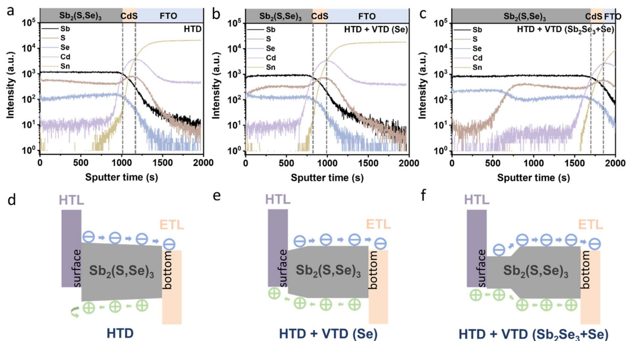
Fig. 4 Depth profiling via TOF-SIMS of the \text{Sb}_2(\text{S},\text{Se})_3 films and energy band structures of the corresponding solar devices: (a and d) HTD, (b and e) HTD + VTD (Se), and (c and f) HTD + VTD ( \text{Sb}_2\text{Se}_3 + \text{Se} ).
