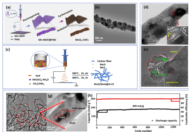
Fig. 5 (a) Schematic illustration of the synthesis process and (b) TEM image of \text{MnO}_x\text{-CNFs} . Adapted from ref. 31, copyright 2022, American Chemical Society. (c) An illustration of the \text{MnS/MnO@N-CF} synthesis process. (d) SEM and (e) TEM images of \text{MnS/MnO@N-CF} . Adapted from ref. 27, copyright 2022, Elsevier B.V. (f and g) TEM images of \text{Mn}_3\text{O}_4\text{@HCFs} . (h) Long cycling performance and coulombic efficiency of the \text{Mn}_3\text{O}_4\text{@HCF} electrode at 0.4 \text{ A g}^{-1} . Adapted from ref. 59, copyright 2020, Elsevier Ltd.
