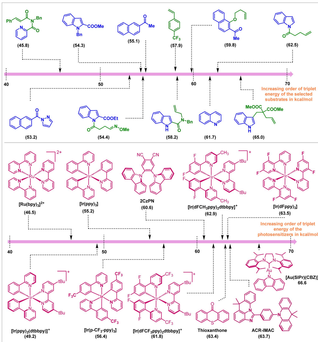
Fig. 16 Photocatalytic dearomative cycloaddition reactions. The figure shows the triplet energies ( E_T ) in kcal mol -1 for various substrates and photosensitizers. The substrates are arranged in two rows, and the photosensitizers are arranged in two rows. The energy levels are indicated by arrows pointing to a scale from 40 to 70 kcal/mol. The note indicates 'Increasing order of triplet energy of the selected substrates in kcal/mol' and 'Increasing order of triplet energy of the photosensitizers in kcal/mol'.
