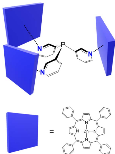
Fig. 1 First example of a \{[P(3\text{-py})_3] \cdot (\text{ZnTPP})_3\} assembly.
