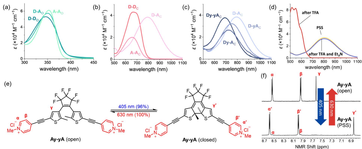
Fig. 3 Absorption spectra of (a) open-form and (b) closed-form D-D , A-A and D-A in MeCN. (c) Absorption spectra of closed-form D-A , Dy-yA , Dy-yA and Dy-yA in MeCN. (d) Absorption spectra of D-A at PSD in MeCN (yellow), MeCN + 0.5% TFA (red), and MeCN + 0.5% TFA + excess Et 3 N (blue). (e) Photoswitching process of the chloride salt of Ay-yA in water triggered by 405 nm light. (f) 1 H NMR spectra showing the reversible switching of Ay-yA (chloride salt) in D 2 O between open-form and the PSS containing 96% closed-form.
