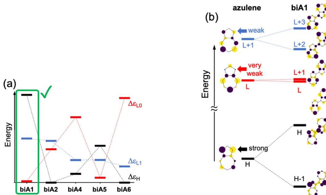
Fig. 3 (a) Orbital energy differences ( \Delta\epsilon_H , \Delta\epsilon_{L1} , and \Delta\epsilon_{L0} ) for symmetrical biazulenes ( biA1 – biA6 ). (b) Molecular orbital diagrams of azulene and biA1 . Participation of p_z -orbital in position 1 of azulene highlighted. Energy gaps and orbitals obtained with the Hückel model. H = HOMO; L = LUMO.
