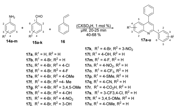
Scheme 6 Synthesis of various derivatives of quinolines 17a–u.
