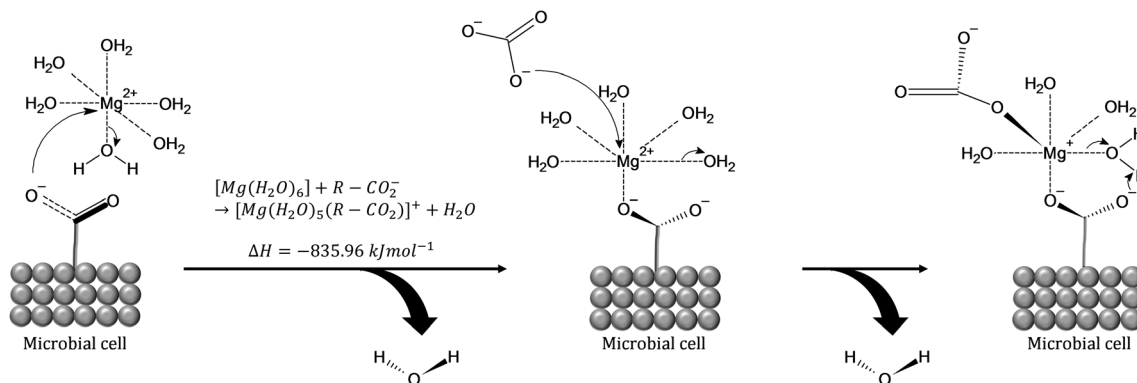
Fig. 6 (1) [\text{Mg}(\text{H}_2\text{O})_6]^{2+} attracted to carboxyl group on a microbial cell wall. (2) The complex attaches to the carboxyl group and ejects one hydration water in an energetically favorable reaction (inserted equation). The new [\text{Mg}(\text{H}_2\text{O})_5(\text{R}-\text{CO}_2)]^+ complex carries a residual positive charge that is satisfied by the inclusion of aqueous carbonate ( \text{CO}_3^{2-} ) or bicarbonate ( \text{HCO}_3^{2-} ). 42 Drawn with the ACD (ChemSketch (freeware) v. 2018.1.1).
