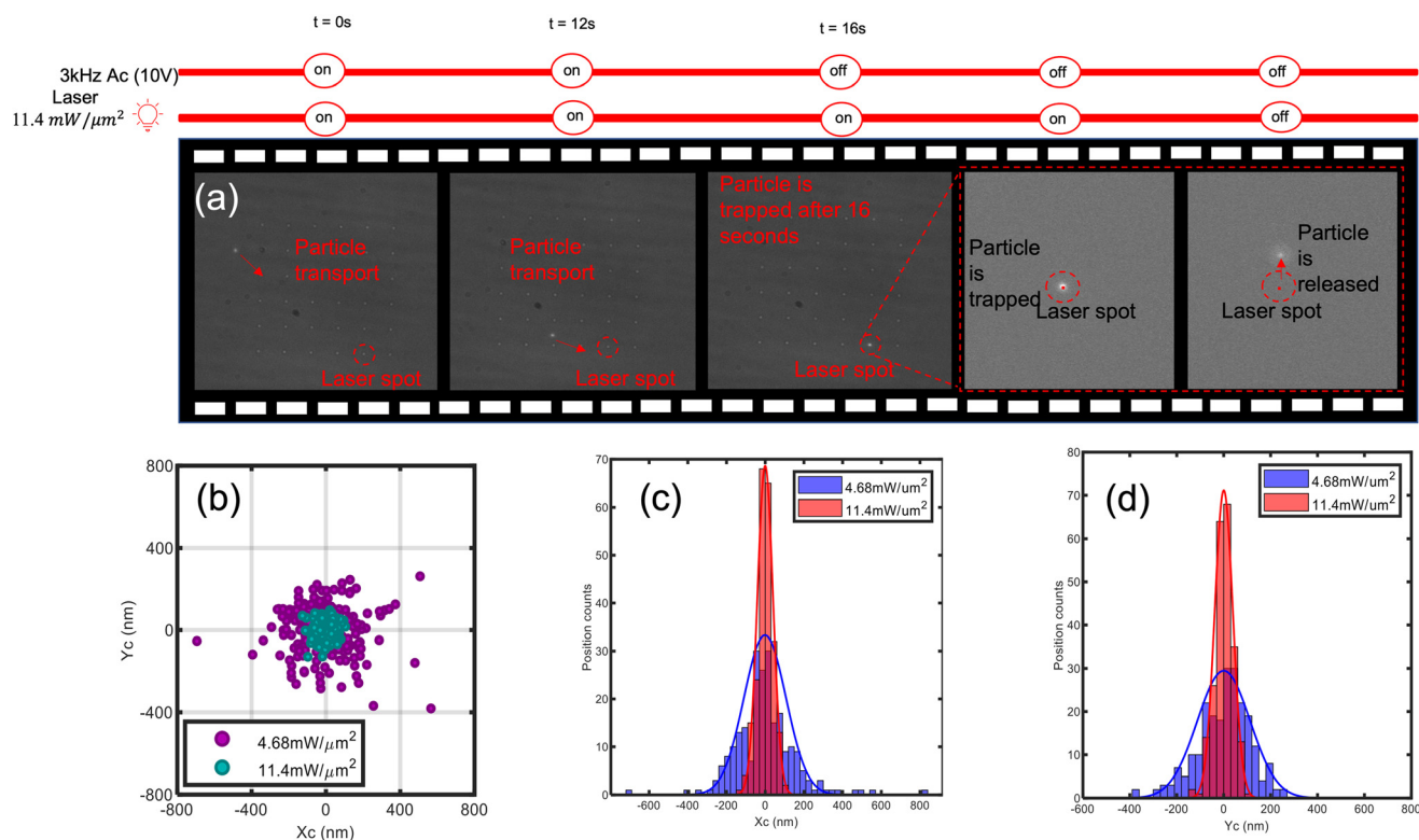
Fig. 5 ETP transport and trapping of a 25 nm polystyrene particle. (a) ETP transport of a 25 nm polystyrene bead from a distance 63 \mu\text{m} away within 16 seconds under an AC voltage of 10 V and 3 kHz frequency. The particle remains trapped at the hotspot after the AC voltage is turned off and gets released after the trapping laser is turned off. (b) Particle position plot for a 25 nm polystyrene bead trapped at the plasmonic hotspot for two different laser intensities. This shows increased particle localization at higher laser intensities, where X_c and Y_c represent the centre of the particle. (c) Particle position histograms for the position of the particle in (b) along the X axis for two different laser intensities. (d) Particle position histograms for the position of the particle in (b) along the Y axis for two different laser intensities.
