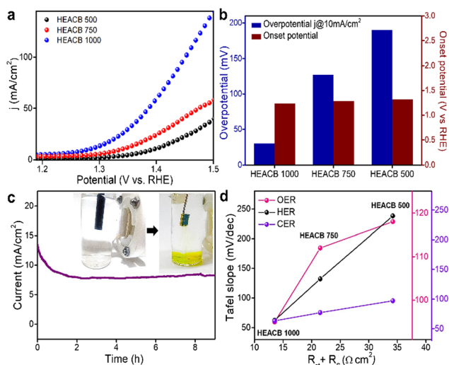
Fig. 5 (a) LSV curves of HEACB samples in the CER polarization region in 0.5 M H 2 SO 4 and 4 M NaCl. (b) Comparison plot of onset and overpotential of HEACB samples. (c) Chronoamperometry test for HEACB 1000 at room temperature in the CER polarization potential, and (d) Tafel slope plot comparing HEACB samples with system resistance derived from electrochemical impedance spectroscopic analysis.
