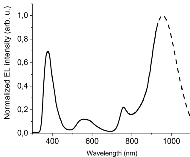
Fig. 5 EL at 100 mA cm -2 of ITO/PEDOT:PSS/PVK/40% F8BT: 10% F8BT-TTBT: 50% DTDAP/TPBi/Ba/Al device. Dashed line shows simulated extrapolation of the spectrum.
