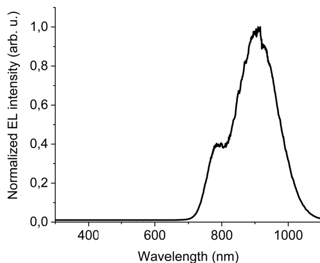
Fig. 6 EL at 100 mA cm -2 of ITO/ZnO/PEIE/40% F8BT: 10% F8BT-TTBT: 50% DTDAP/CBP/Au inverted architecture device.
