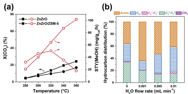
Fig. 9 (a) The hydrogenation of \text{CO}_2 over ZnZrO and ZnZrO/HZSM-5. (b) Ethene conversion over HZSM-5 with co-feeding different contents of \text{H}_2\text{O} . 47 Reproduced from ref. 47 with permission from Elsevier, copyright 2019.
