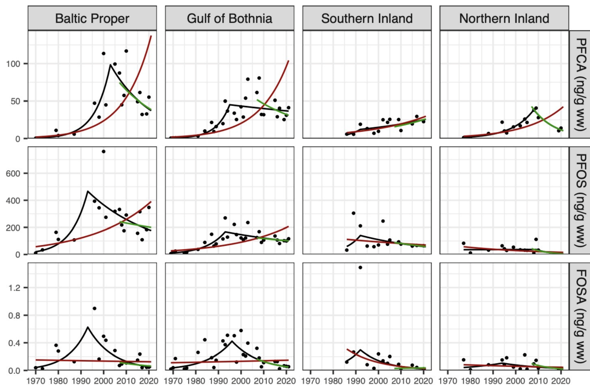
Fig. 3 Change-point graphs for the summed concentration of PFCAs, PFOS and FOSA across the four sampling regions. Each dot represents a yearly geometric average. Change-point trends are provided in black, while log-linear trends for the whole period and last 15 years are shown in red and green, respectively. Statistical significance is provided in Table 1.
