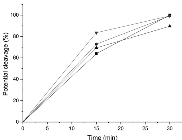
Fig. 11 Potential conversion of the \beta\text{-O-4'} ( \beta ) ( \blacksquare ), \beta\text{-O-4'} ( \alpha ) ( \bullet ), \beta\text{-5'} ( \blacktriangle ) and 5\text{-5'} ( \blacktriangledown ) environments according to the HMBC spectra with the integration of the signals at (4.19, 146.77 ppm), (4.97, 108.42 ppm), (5.08, 110.29 ppm) and (6.89, 124.09 ppm) respectively.
