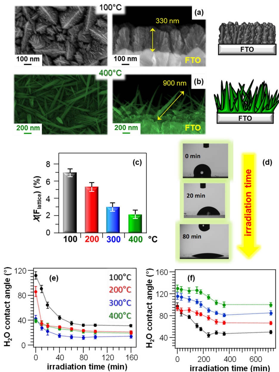
Fig. 13 Chemico-physical and functional characterization of \text{MnO}_2 -based nanomaterials fabricated on FTO substrates via PE-CVD at different temperatures, starting from a fluorinated \text{Mn(II)} diamine diketone precursor. (a and b) Representative plane-view (left) and cross-sectional (right) SEM images for samples grown at 100 and 400 °C, along with sketches modelling the morphological evolution from hierarchical dendritic structures to quasi-1D nanosystems. (c) Lattice fluorine contribution, measured by XPS, as a function of the growth temperature. X(F_{\text{lattice}}) was calculated from atomic percentages (%at) as (\% \text{at } F_{\text{lattice}}) \times 100 / [(\% \text{at } F_{\text{lattice}}) + (\% \text{at } \text{Mn})] . 44 (d) Photographs of \text{H}_2\text{O} droplets on a specimen fabricated at 100 °C after UV irradiation for different times. (e) PH and (f) PCO performances of \text{MnO}_2 -based nanomaterials: water contact angle vs. irradiation time for as-prepared (e) and methyl stearate-coated systems (f). Reproduced with permission from ref. 44. Copyright 2019, The Royal Society of Chemistry.
