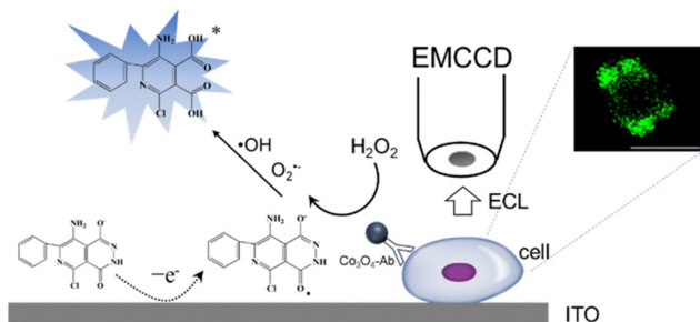
Scheme 1 ECL mechanism based on the \text{Co}_3\text{O}_4 nanzyme for CEA antigen imaging at the cellular membrane.
