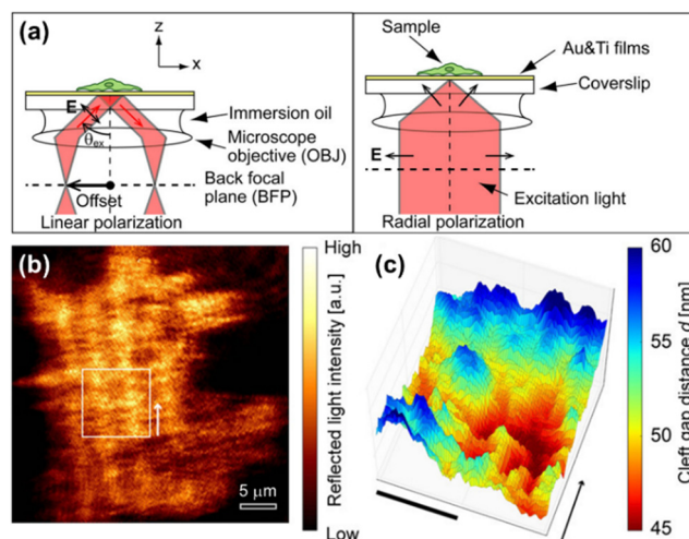
Fig. 3 (a) Schematic illustration of optical paths nearby the sample for lens-imaging-type (LISPM, left) and scanning localized (SLSPM, right) SPRM. (b) Representative LISPM (b) and SLSPM (c) images of HEK293 cells cultured on a poly-L-lysine-coated gold surface. Adapted with permission from ref. 57 (Copyright 2014 American Chemical Society).
