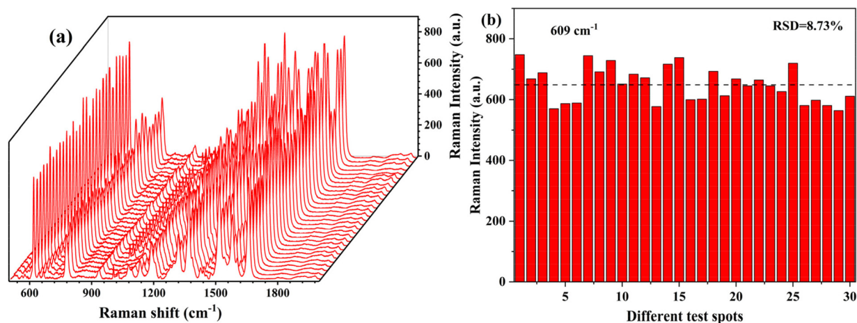
Fig. 3 (a) SERS spectra of and (b) peak intensities at 609 \text{ cm}^{-1} of 10^{-9} M R6G obtained from 30 random points on the same substrate.
