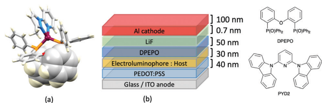
Fig. 15 (a) Structure of the complex cation in [Cu(POP)(3-Meppzpy)] + [BF 4 ] - ·0.5CH 2 Cl 2 (CSD refcode VIZKEW) with Ph ∧ arene π-stacking within the POP ligand shown in space-filling representation. (b) Architecture of solution-processed OLEDs with [Cu(POP)(pzpy)] + [BF 4 ] - derivatives in the active layer. DPEPO = hole-blocking layer; active layer = 20 wt% Cu-iTMC in either DPEPO or PYD2 as host.
