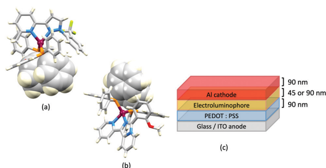
Fig. 16 Structures of the complex cations in (a) [Cu(POP)( 8 )] + [BF 4 ] - ·EtOH (CSD refcode JUFNOP) and (b) [Cu(POP)( 11 )] + [PF 6 ] - showing Ph ∧ arene π-stacking in the POP ligand (space-filling representation). (c) LEC architecture for testing with [Cu(POP)( 11 )] + [PF 6 ] - in the active layer; LECs were driven with a pulsed current.
