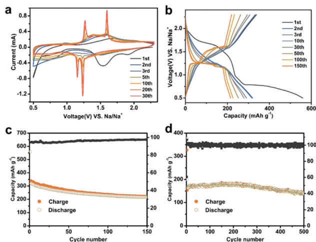
Fig. 7 Electrochemical performance of the Ni-DHBQ electrode recorded in the voltage range of 0.5–2.3 V ( vs. Na/Na + ). (a) CV curves at a scan rate of 0.5 mV s −1 . (b) Discharge–charge voltage profiles of Ni-DHBQ electrodes at 0.1 A g −1 . (c) and (d) Cycling performance of Ni-DHBQ electrodes at a current density of 0.1 A g −1 and 5 A g −1 , respectively.
