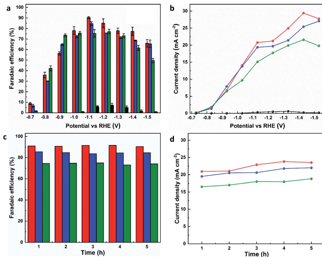
Fig. 3 Catalytic performance of MFM-220-p/CP (red lines or column), MFM-221-p/CP (blue lines or column), MFM-222-p/CP (green lines or column), and CP (black lines or column) electrodes for \text{CO}_2\text{RR} in 0.1 M \text{KHCO}_3 . Plots of (a) \text{FE}_{\text{formate}} vs. potential, (b) current density for formate production vs. potential, (c) \text{FE}_{\text{formate}} vs. time, and (d) current density of formate vs. time for reduction of \text{CO}_2 at -1.1 V vs. RHE.
