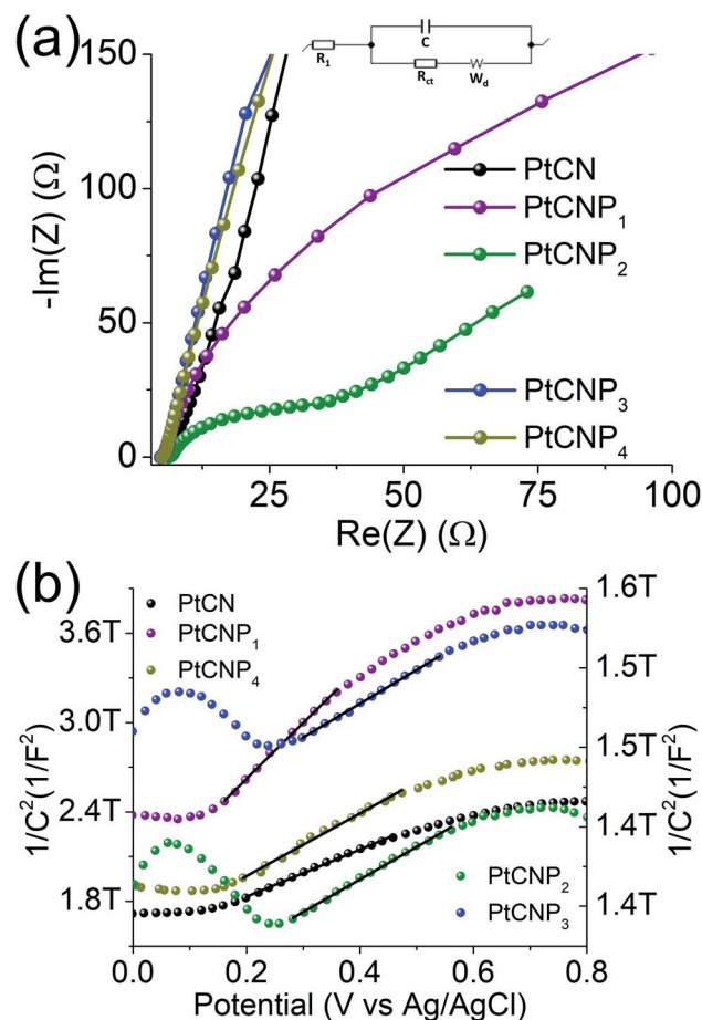
Fig. 6 (a) Nyquist plots for the sample series produced from electrochemical impedance measurements at -10 \text{ mV} overpotential. Inset is the Randle's equivalent circuit where R_1 is the solution resistance, R_{\text{ct}} is the charge-transfer resistance, C is the double-layer capacitance, and W_d is the Warburg diffusion term. (b) Mott–Schottky measurements for the sample series performed in 0.1 M \text{Na}_2\text{SO}_4 . Potentials are vs. an Ag/AgCl reference electrode. Regression taken within the linear portion of each sample is shown as a black solid line. Y-axis on the left correspond to samples PtCN, PtCNP 1 , and PtCNP 4 while y-axis on the right corresponds to PtCNP 2 and PtCNP 3 .
