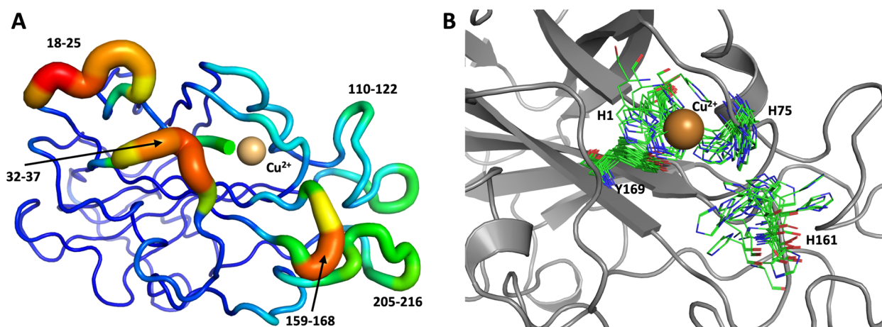
Fig. 10 Conformational flexibility of a related LPMO and active-site residues ( Mt PMO3* PDB 5UFV) results from 1 \mu\text{s} MD simulation. (A) Conformational flexibility of based on RMSF 10 . (B) Active site residues. His161 (equivalent to His157) is highly flexible and transition back and forth between the inward and outward conformations during the 1 \mu\text{s} MD simulation (see Fig. 9 legend for more details).
