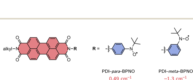
Fig. 3 Structures of the perylene diimide derivatives used for benchmarking and calculated values of J_{\text{TR}} using CASSCF/QD-NEVPT2.
