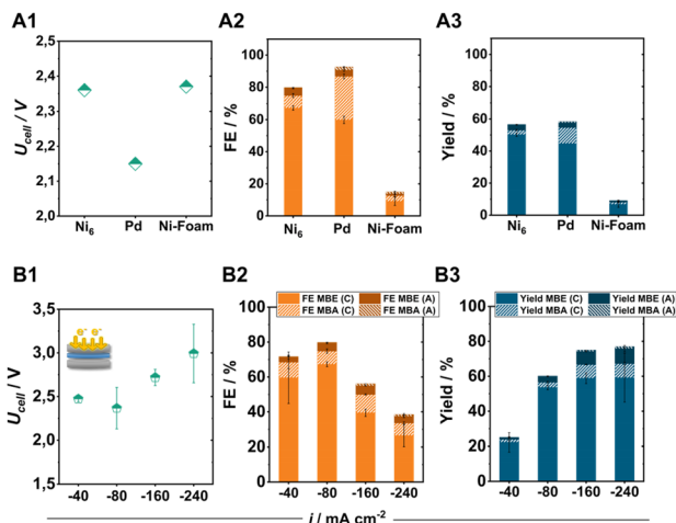
Fig. 5 Comparison of Ni 6 with the typical electrocatalysts for the ECH, Pd and Ni-foam. The obtained cell voltage (A1), faradaic efficiency (A2), and yield (A3) after 2 h of electrolysis at 80 \text{mA cm}^{-2} . Effect of the applied current density on the ECH product distribution for Ni 6 -based electrodes in a zero-gap electrolyser. The obtained cell voltage (B1) faradaic efficiency (B2) and yield (B3) after 2 h of electrolysis at the applied current density. Here, \text{FE}_{\text{MBX}} (C) and \text{FE}_{\text{MBX}} (A) (X: E, A) correspond to the FE values of ECH products detected in the catholyte and anolyte after electrolysis, respectively.
