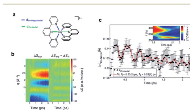
Fig. 15 (a) Chemical structure of [Co(terpy) 2 ] 2+ . The axial and equatorial Co–N bonds, which show anisotropic expansion upon spin state transition from LS to HS induced by 530 nm photoexcitation, are indicated by green and blue lines. (b) Fs-TRXL data ( \Delta S_{\text{exp}} , left) and corresponding fit ( \Delta S_{\text{fit}} , right). (c) Time evolution of the Co–N bond lengths showing coherent wavepacket motions of [Co(terpy) 2 ] 2+ . The inset shows a time-resolved Fourier transform of the oscillatory component of the fs-TRXL signal in (b), which shows a sequential activation of two vibrational modes. A heuristic fit is shown in solid red line incorporating sequential activation of two vibrational modes: one showing a breathing motion (period of \sim 0.33 ps) and the other showing a pincerlike movements (period of \sim 0.23 ps). Reproduced from ref. 61 with the permission of the American Physical Society, copyright 2016.
