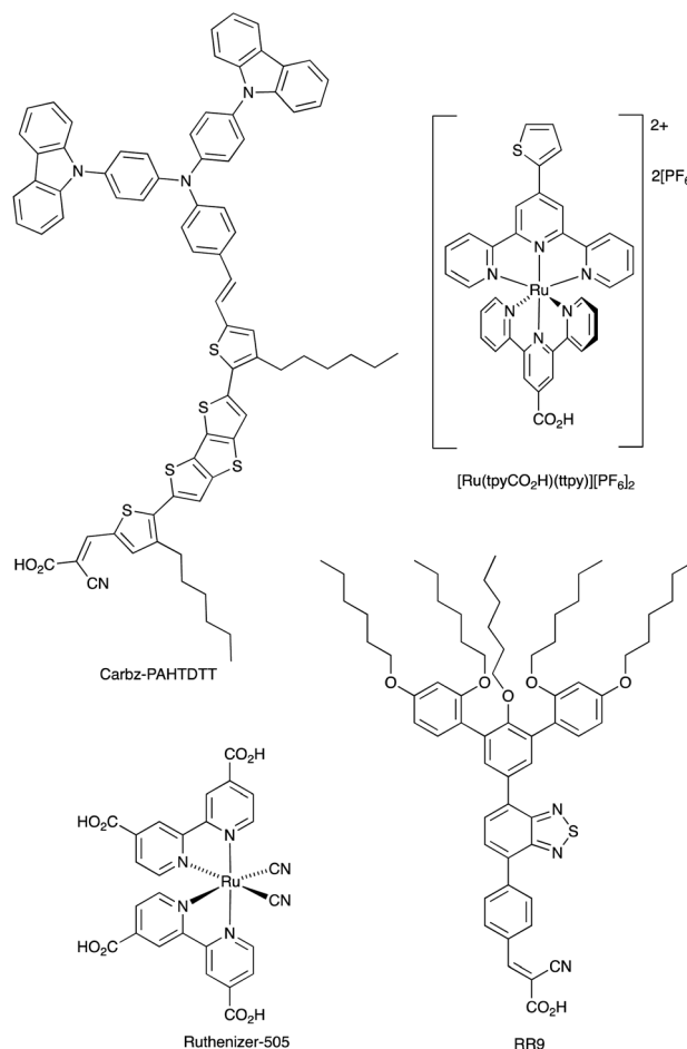
Scheme 12 Structures of the metal-free dyes Carbz-PAHTDIT and RR9, and the ruthenium(II) dyes [\text{Ru}(\text{tpyCO}_2\text{H})(\text{ttpy})][\text{PF}_6]_2 (tpy = 2,2':6',2''-terpyridine) and the commercially available Ruthenizer-505.
