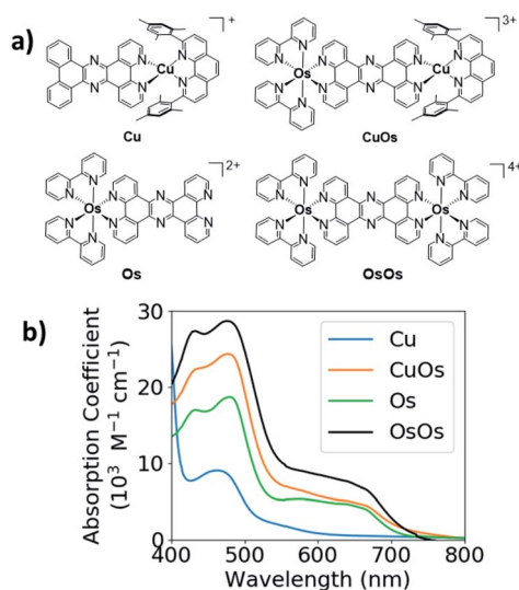
Fig. 1 (a) Structures of Os, Cu, CuOs, and OsOs; (b) UV-vis spectra of Os, Cu, and CuOs and OsOs.
