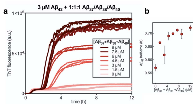
Fig. 11 (a) The aggregation of 3 μM Aβ 42 with varying concentrations of a 1 : 1 : 1 mixture of Aβ 37 /Aβ 38 /Aβ 40 . (b) The half-time of the aggregation of Aβ 42 shown in (a) versus the total concentration of the three shorter alloforms. Kinetic experiment was performed in 20 mM sodium phosphate buffer, pH 7.4, with 200 μM EDTA, 0.02% NaN 3 , and 20 μM ThT.
