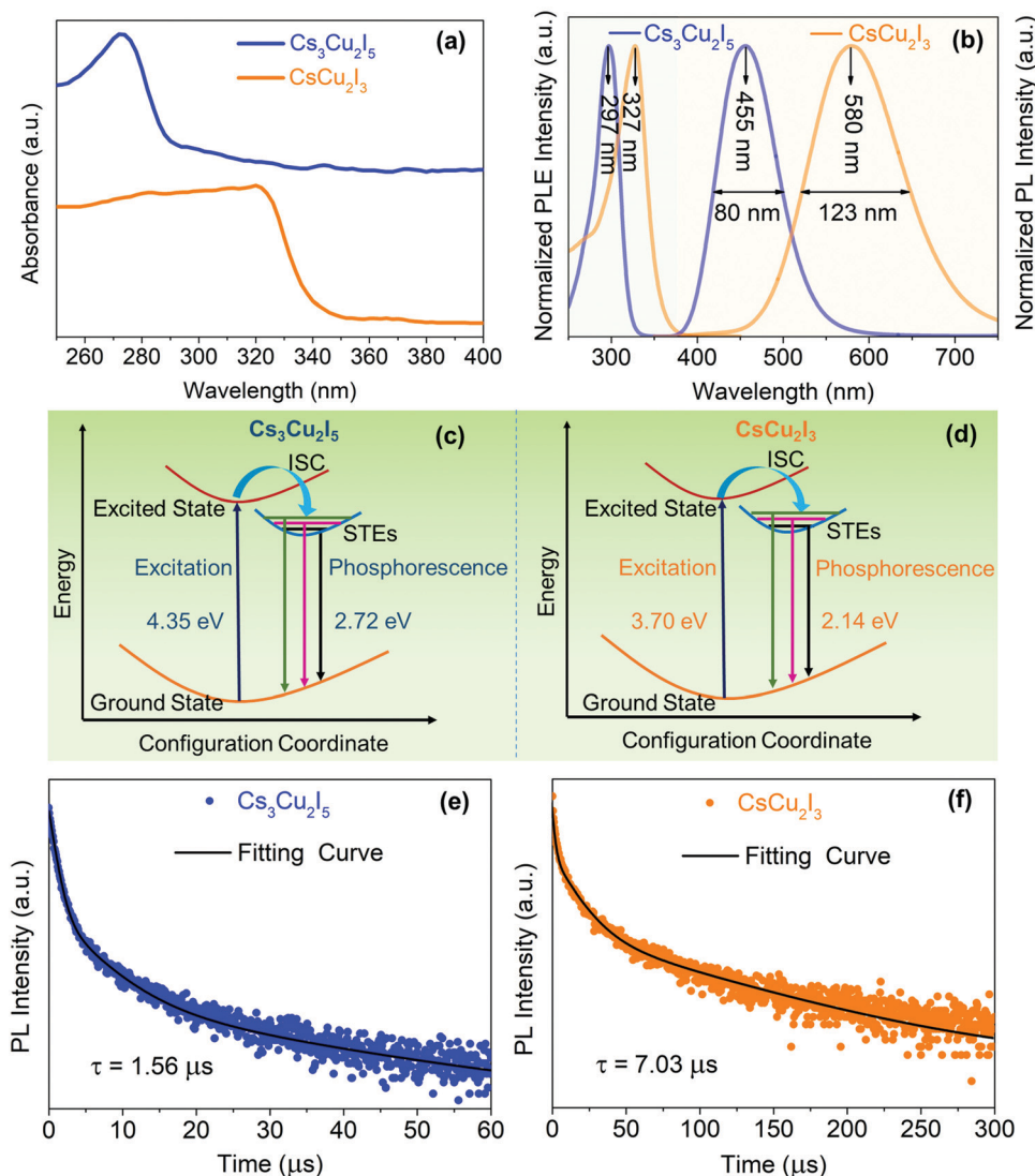
Fig. 3 (a) UV-vis absorption spectra of Cs 3 Cu 2 I 5 and CsCu 2 I 3 . (b) PLE and PL spectra of Cs 3 Cu 2 I 5 and CsCu 2 I 3 . Schematic diagram of the STE emission of (c) Cs 3 Cu 2 I 5 and (d) CsCu 2 I 3 . Time-resolved PL decay spectra of (e) Cs 3 Cu 2 I 5 and (f) CsCu 2 I 3 .
