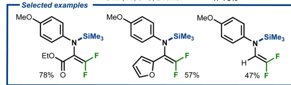
of Fig. 21 Electroreductive defluorinative silylation of trifluoromethyl ketones. 73
