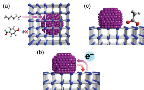
Fig. 4 Schematic illustrations of support effects in heterogeneous catalysis, regarding (a) molecular sieving, (b) charge transfer, and (c) substrate adsorption, which are illustrated with porous MOFs as the support materials.
