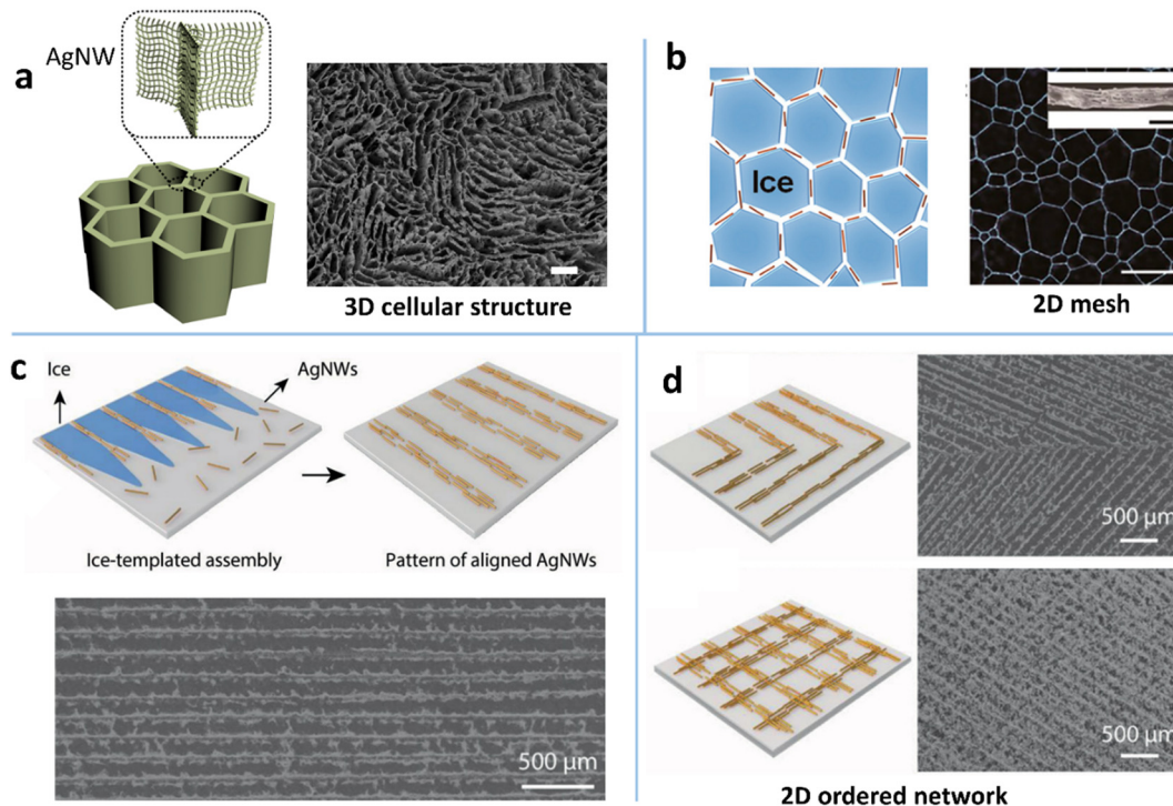
Fig. 3 (a) Illustration of the structure of 3D ice-templating AgNWs and the corresponding SEM image. Reproduced with permission. 109 Copyright 2018, Springer Nature. (b) Schematic of the 2D recrystallized ice template method and the optical microscope (OM) image of the assembled 2D AgNW mesh. Reproduced with permission. 131 Copyright 2017, American Chemical Society. (c) Schematic of the 2D ice-templating method for ordering and patterning AgNWs and the corresponding SEM image. (d) Schematic and SEM images of '>' shaped and orthogonally aligned AgNW patterns fabricated by the 2D ice-templating approach. Reproduced with permission. 36 Copyright 2021, WILEY-VCH.
