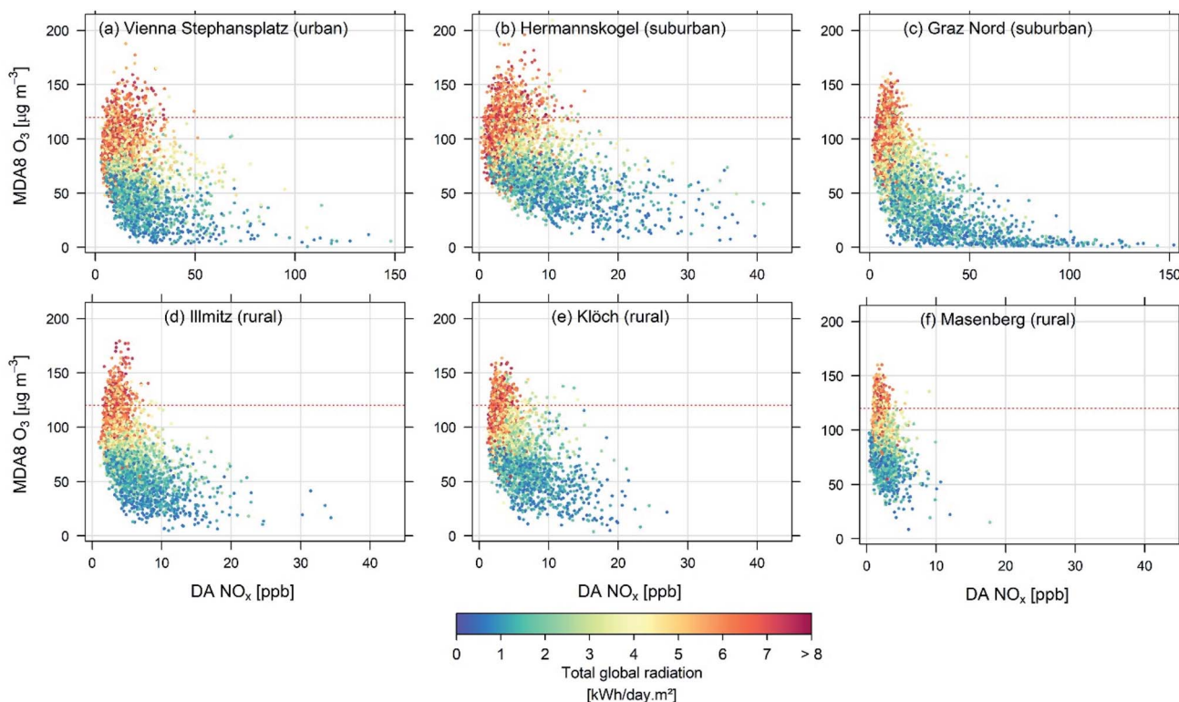
Fig. 4 Scatterplots of MDA8 O 3 versus DA NO x for (a) the urban station Vienna Stephansplatz, (b and c) suburban sites Hermannskogel and Graz Nord, and (d–f) rural sites Illmitz, Klöch, and Masenberg for 2010–2019. The red dotted line in all panels indicates the MDA8 O 3 threshold value of 120 μg m -3 . Colour coding is according to daily total global radiation abundances.
