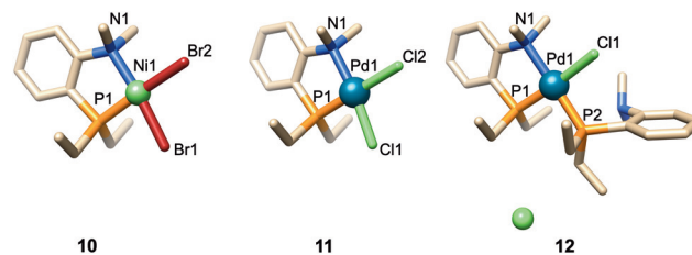
Fig. 3 Single crystal X-ray structures of cavity-free Pd complexes 11 and 12 as well as Ni complex 10 . Solvent molecules have been omitted for clarity. Selected bond lengths (Å) and angles ( ^\circ ): 10 , Ni1–P1 2.1248(10), Ni1–N1 2.010(3), Ni1–Br1 2.3122(6), Ni1–Br2 2.3626(5); P1–Ni1–N1 88.63(9), P1–Ni1–Br1 85.25(3), N1–Ni1–Br2 94.48(8), Br1–Ni1–Br2 91.64(2); 11 , Pd1–P1 2.1857(9), Pd1–N1 2.111(3), Pd1–Cl1 2.2982(9), Pd1–Cl2 2.4087(9); P1–Pd1–N1 86.68(8), P1–Pd1–Cl1 87.20(3), N1–Pd1–Cl2 94.33(8), Cl1–Pd1–Cl2 91.81(3); 12 , Pd1–P1 2.2326(15), Pd1–P2 2.2724(14), Pd1–N1 2.185(5), Pd1–Cl1 2.3728(14); P1–Pd1–N1 84.71(17), P1–Pd1–P2 95.45(5), N1–Pd1–Cl1 91.36(17), P2–Pd1–Cl1 88.28(5).
